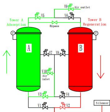
FIG.1 Tower A adsorption, tower B regeneration
